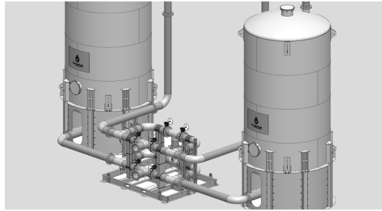
H2S Removal
