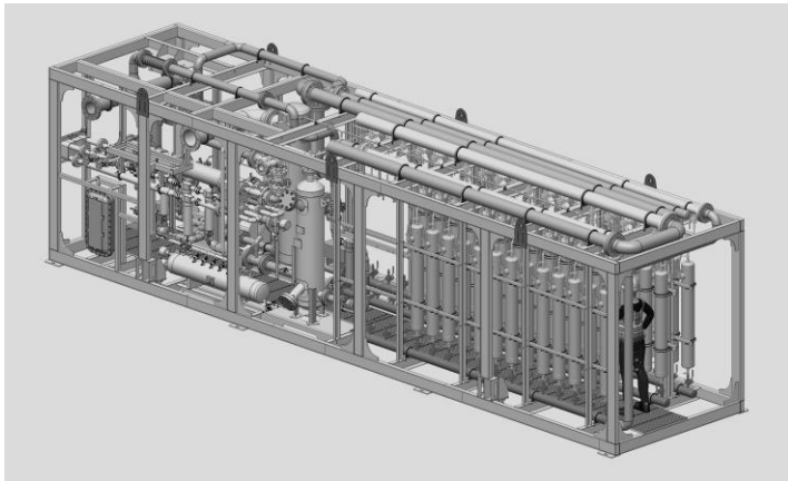
Biogas Membrane Separation
